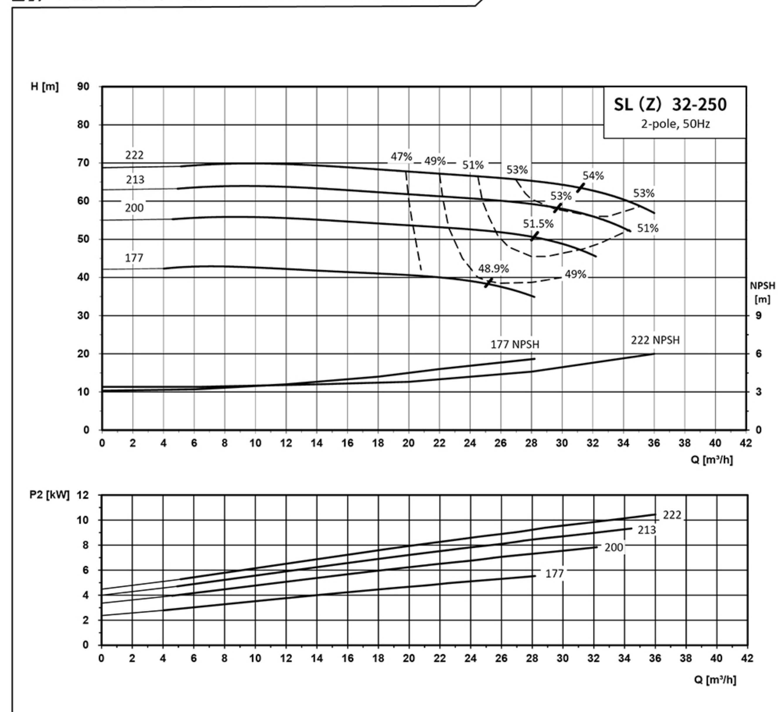
性能曲线和技术数据 Performance Curves and Technical Data
