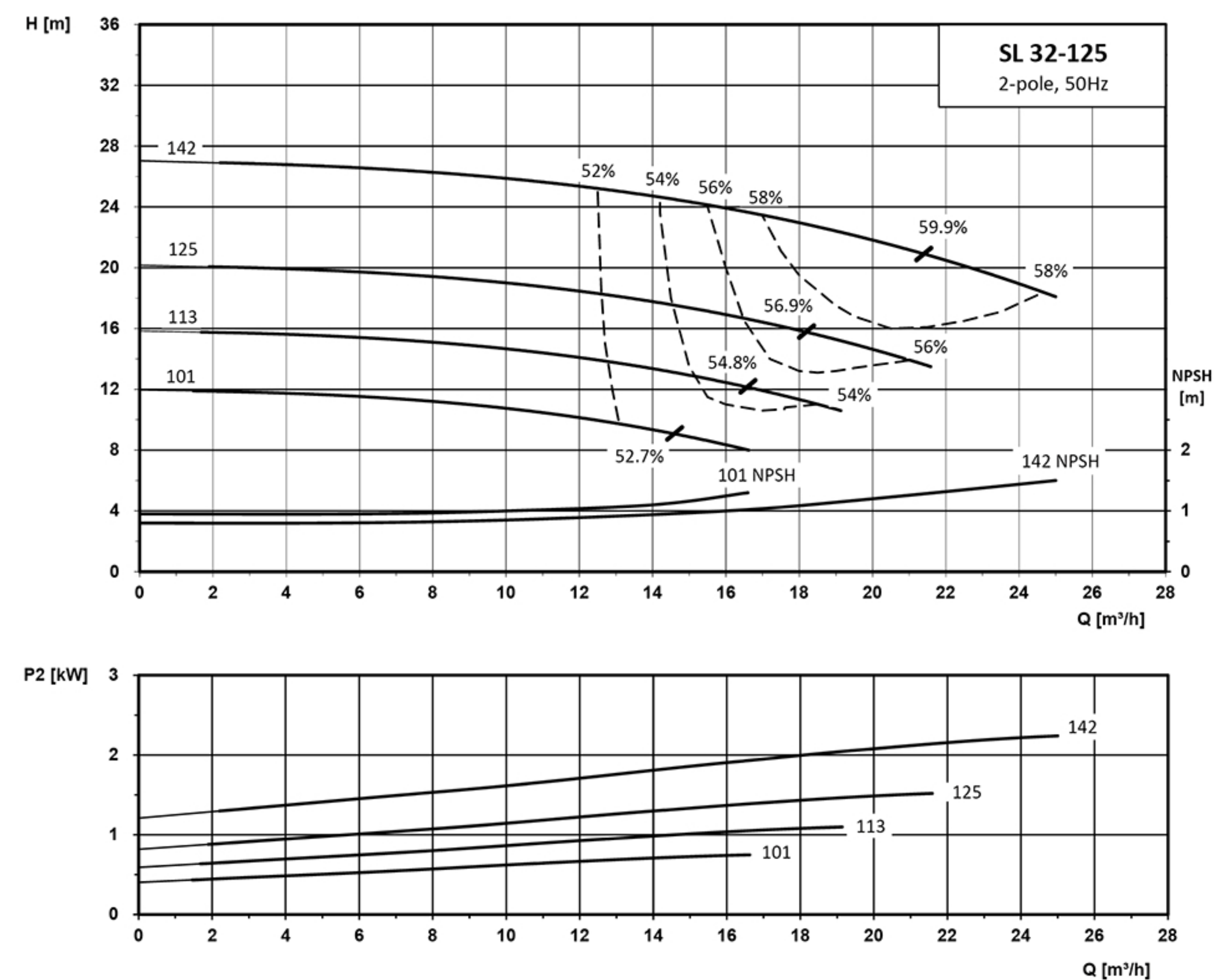
性能曲线和技术数据 Performance Curves and Technical Data
